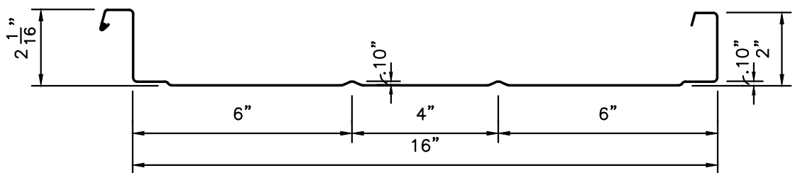
216 Roof Panel With Beaded Pan
