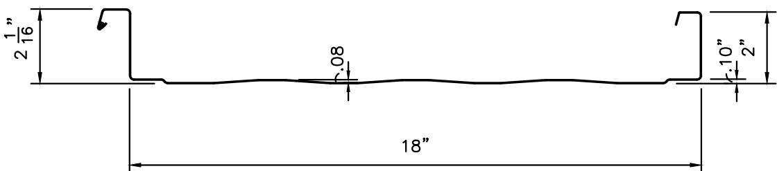
218 Roof Panel With Striated Pan
