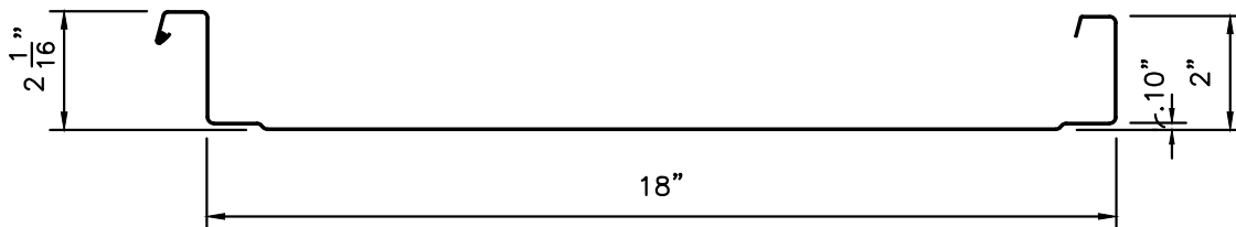
218 Roof Panel With Flat Pan
