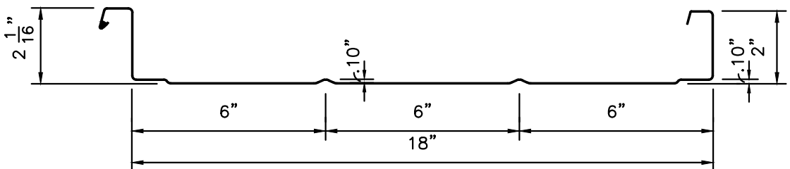
218 Roof Panel With Beaded Pan
