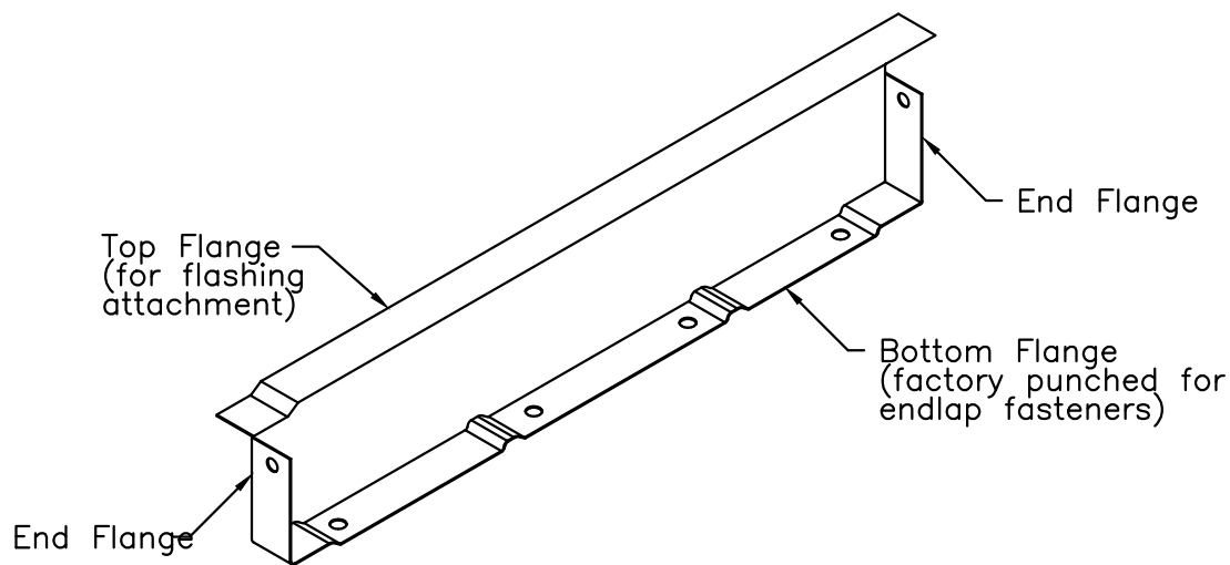
End Dam – Inside View
