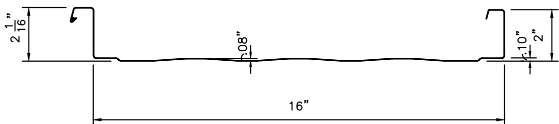
216 Roof Panel With Striated Pan
