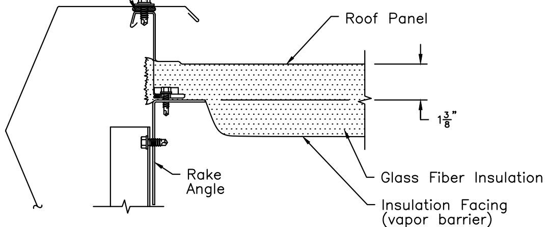
Section @ Rake
