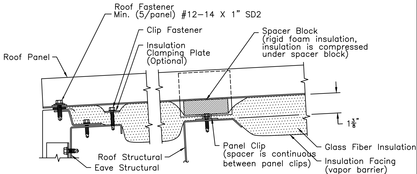
Section @ Structural
